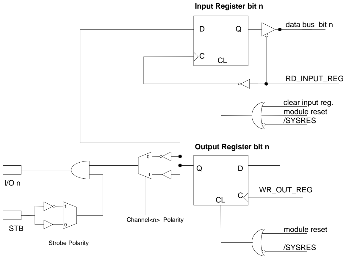
fig 3. 4 : Channel<n> configured as Input, Externally Strobed.
