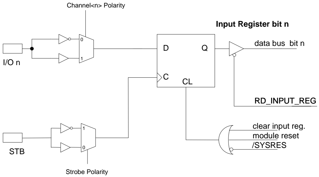
fig 3. 4 : Channel<n> configured as Input, Externally Strobed.
