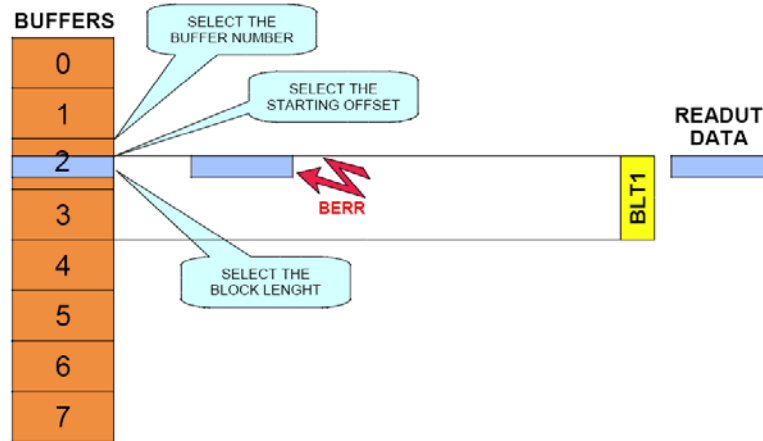
Fig. 3.24: Example of random readout
