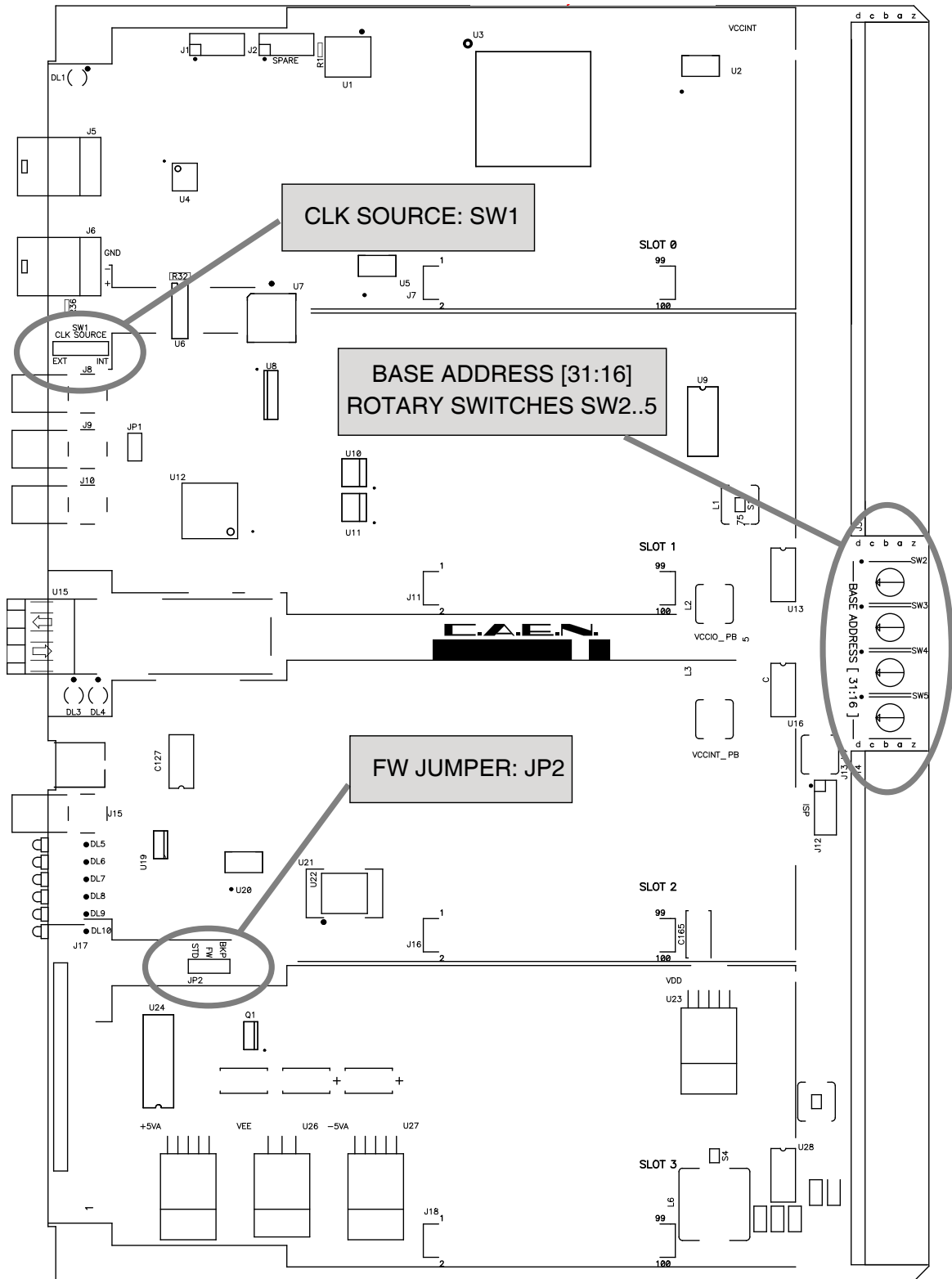
Fig. 2.3: Rotary and dip switches location
