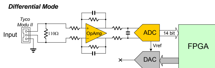
Fig. 3.2: Differential input diagram
