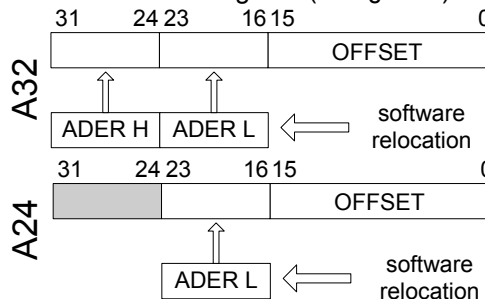
Fig. 3.22: Software relocation of base address
