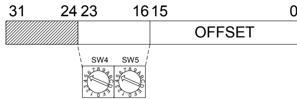
Fig. 3.19: A24 addressing
