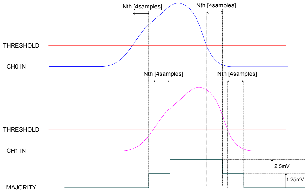
Fig. 3.15: Majority logic (2 channels over threshold; bit[6] of Ch. Config. Register =0)
