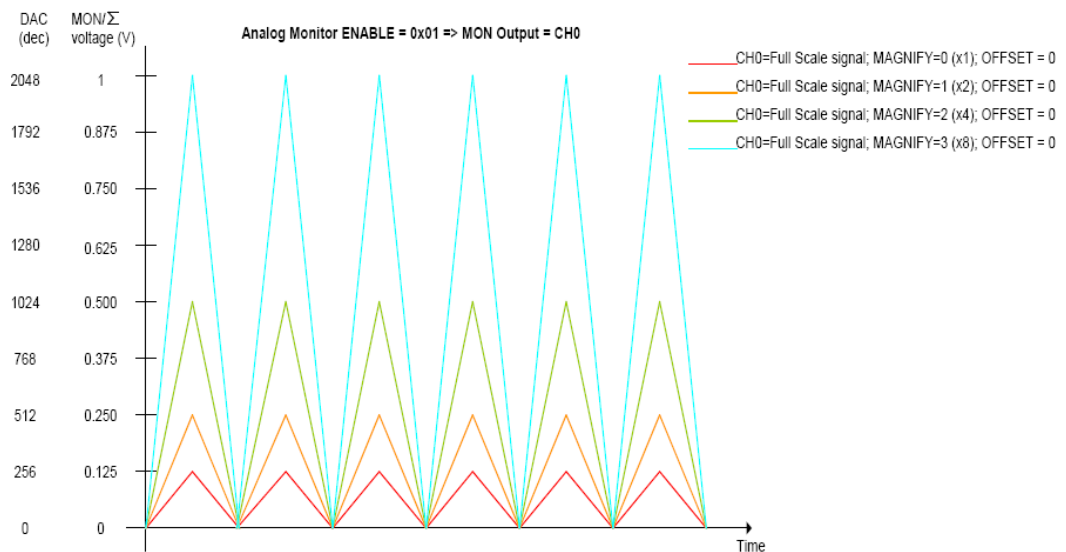
Fig. 3.17: Example of Magnify parameter use on single channel
