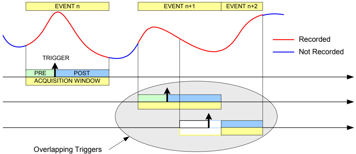
Fig. 3.7: Trigger Overlap
