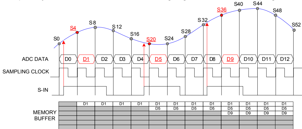
Fig. 3.6: Data storage 2 in Sample Mode
