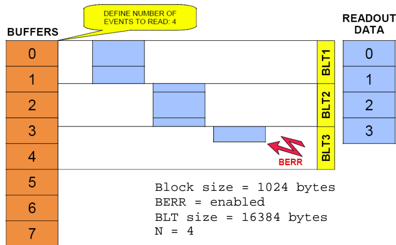
Fig. 3.23: Example of BLT readout
