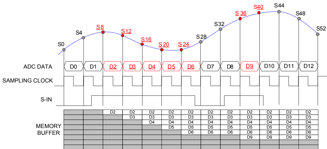
Fig. 3.5: Data Storage 1 in Gate mode
