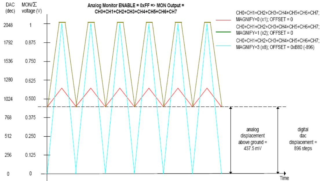
Fig. 3.18: Example of Magnify and Offset parameters use on single channel
