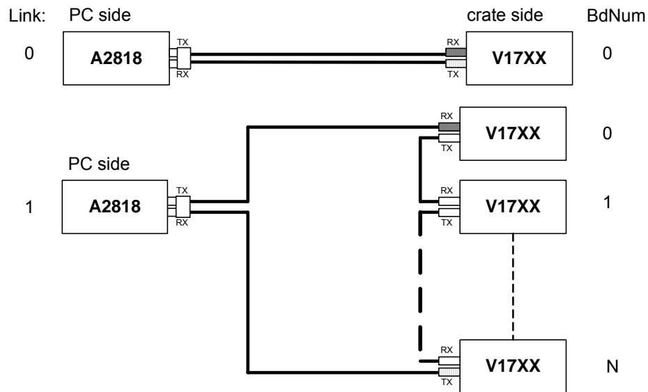
Fig. 3.25: Optical Link daisy chain
