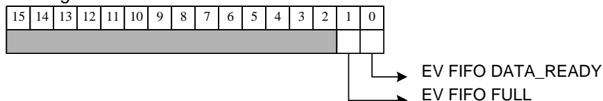
Fig. 6.32: Event FIFO Status register
